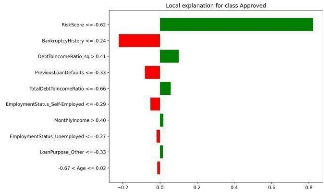
Fig. 11. LIME Approved
