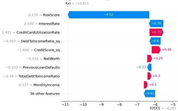
Fig. 9. SHAP Approved
