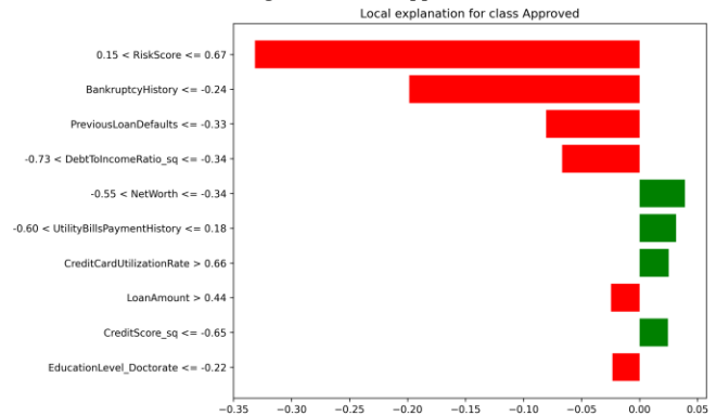
Fig. 11. LIME Approved
