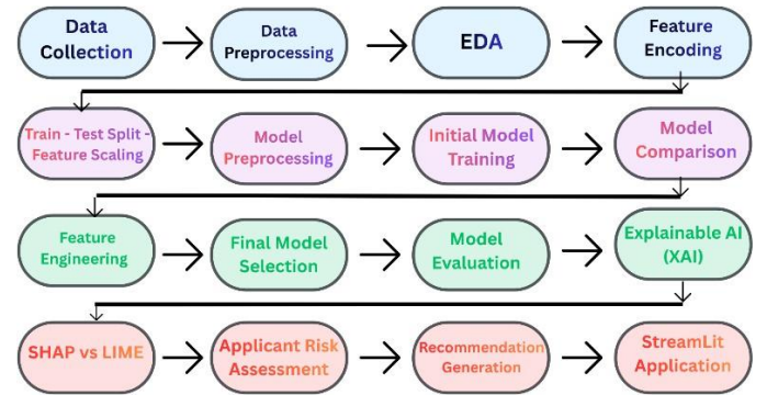
Fig. 1. Methodology Flow
